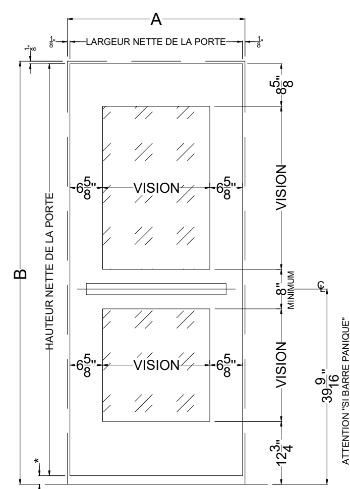
PORTE ELEVATION 2BH
