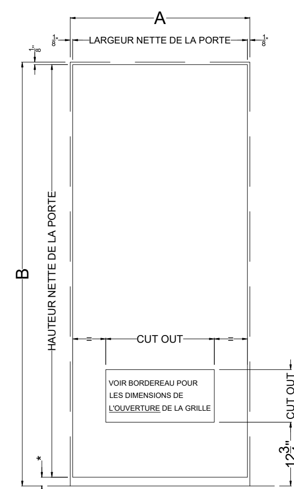
PORTE ELEVATION BGR
