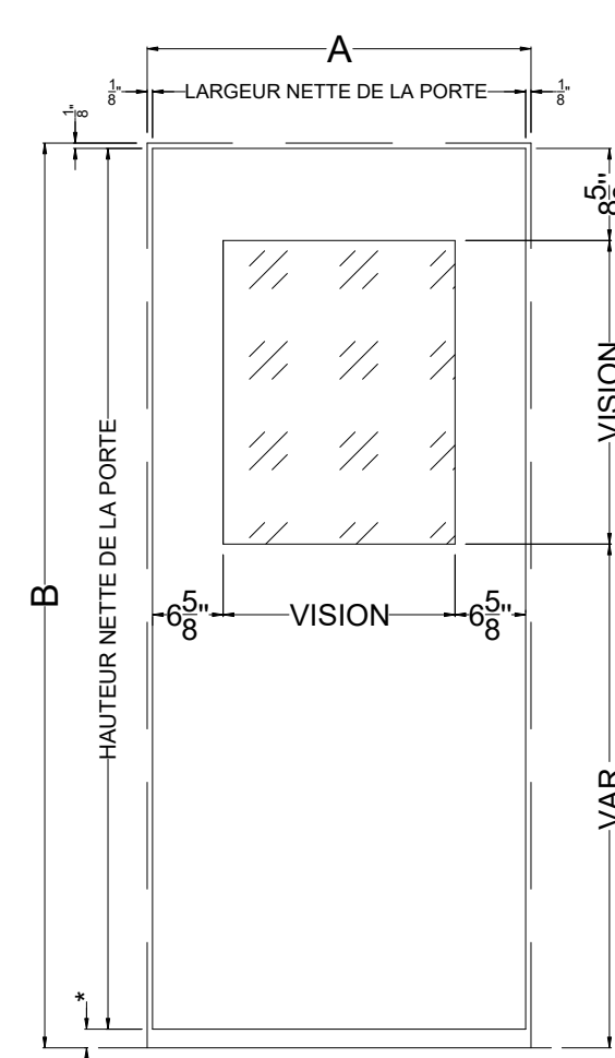
PORTE ELEVATION BH
