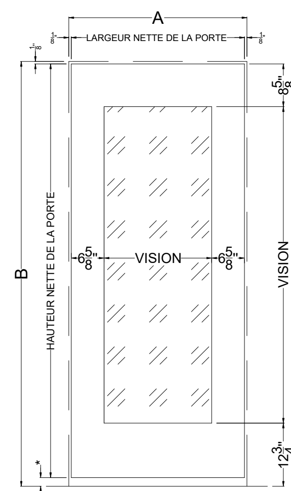
PORTE ELEVATION BFG
