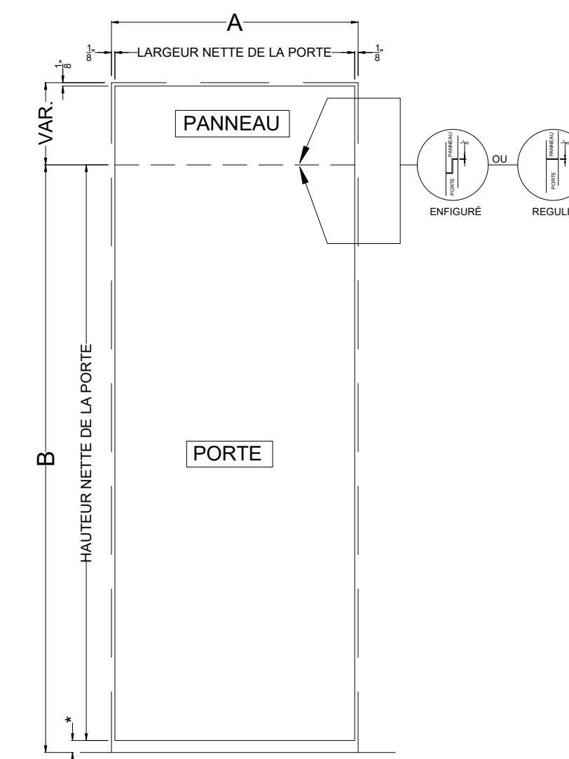
PORTE ELEVATION BFP
