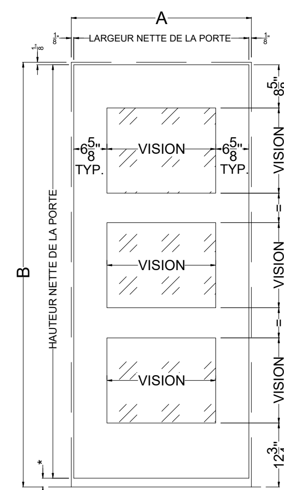
PORTE ELEVATION B3V
