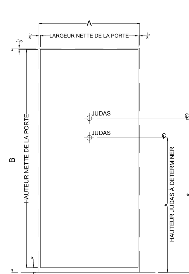
PORTE ELEVATION J2 (LOGEMENT ADAPTABLE)
