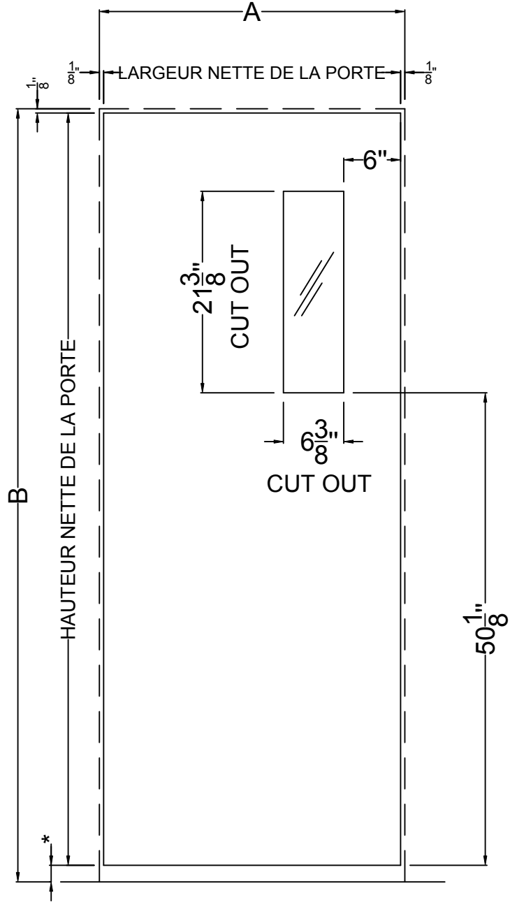
PORTE ELEVATION NLH
