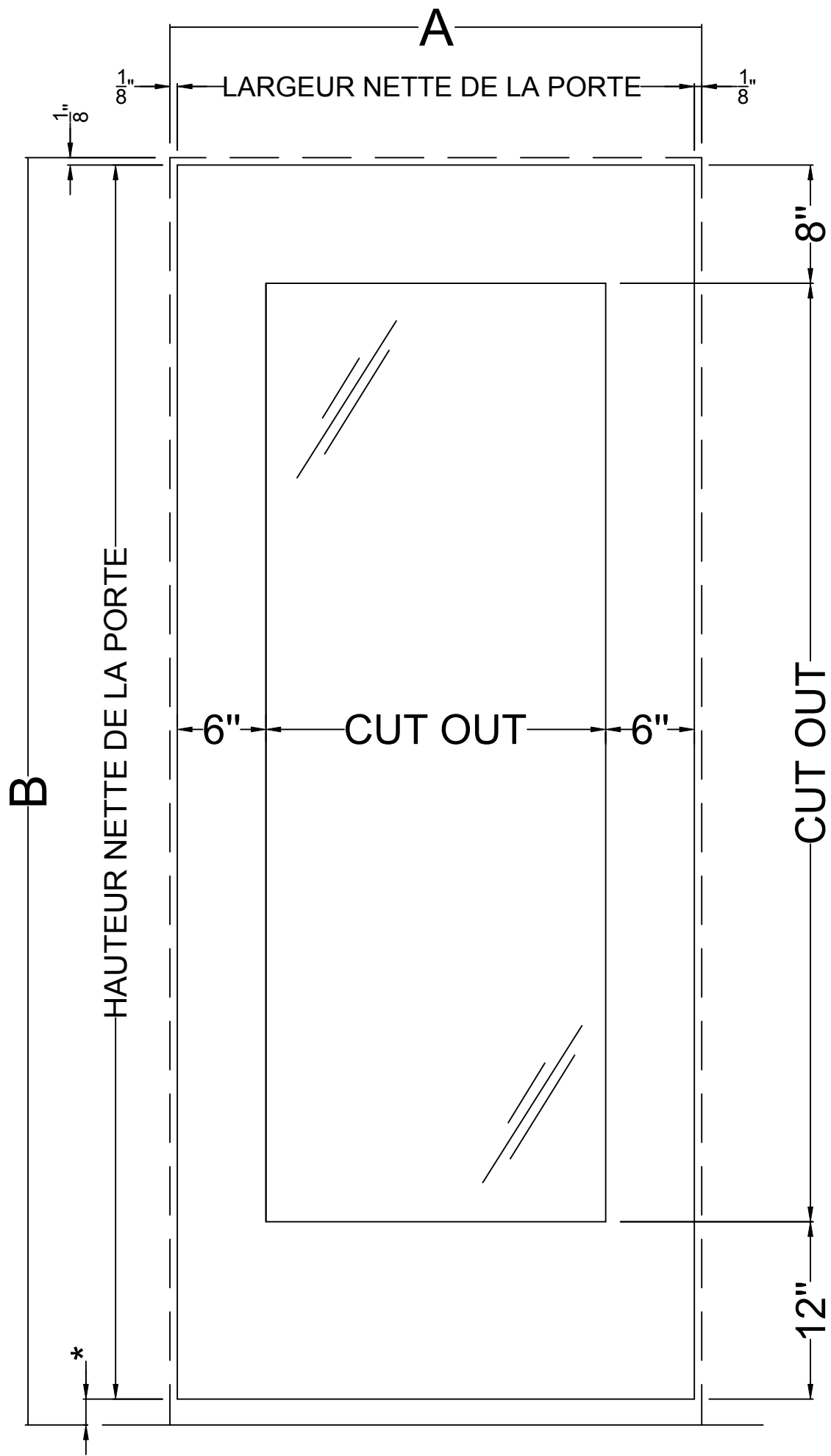
PORTE ELEVATION FG
