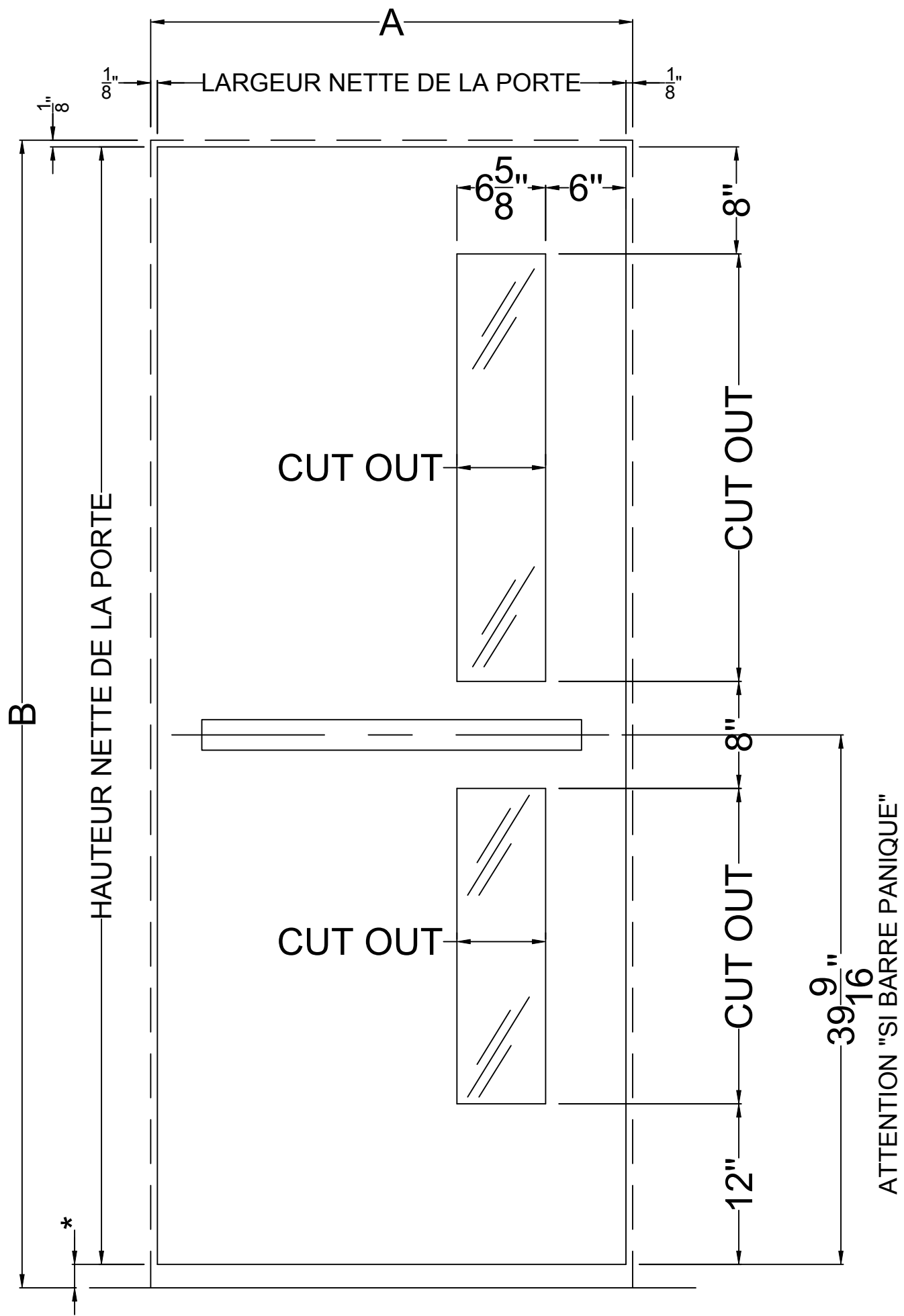
PORTE ELEVATION 2NL
